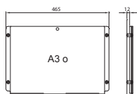
WS-LED A3o
