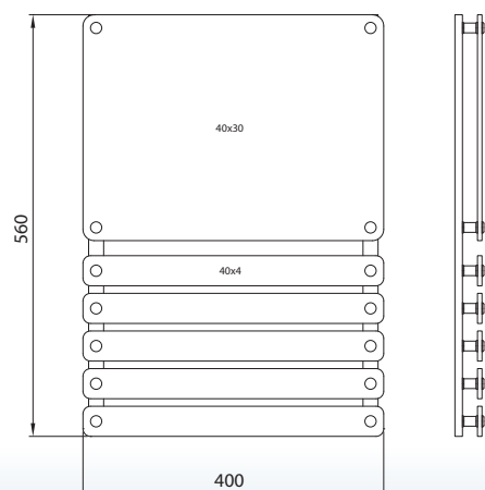
RAIL-TAPWS 40x30 5-40x4
