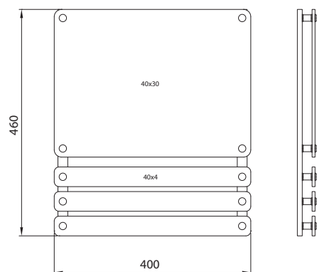
RAIL-TAPWS 40x30 3-40x4
